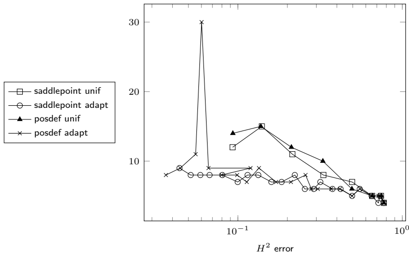
FIGURE 6. Comparison of semismooth Newton iterations in Experiment 2 dependent on the H^2 error; saddle-point formulation (saddlepoint) and positive definite formulation (posdef).
