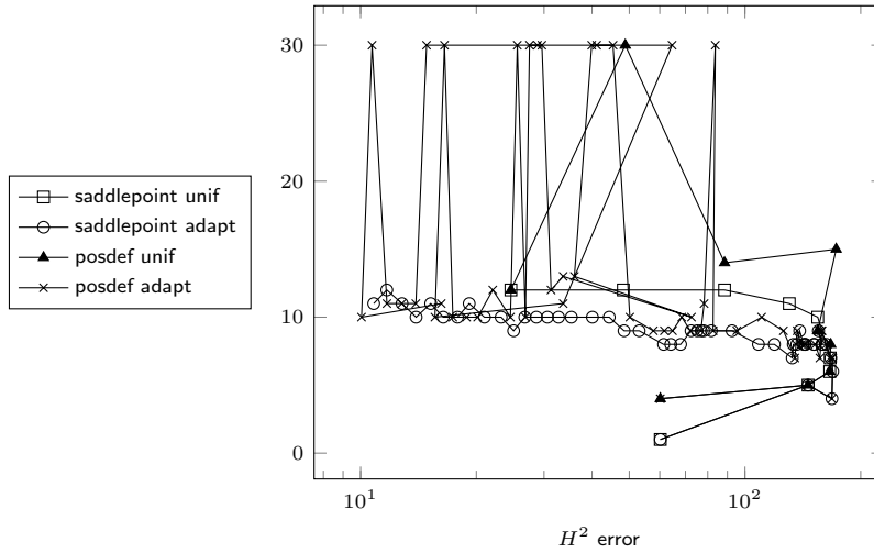
FIGURE 5. Comparison of semismooth Newton iterations in Experiment 1 dependent on the H^2 error; saddle-point formulation (saddlepoint) and positive definite formulation (posdef).
