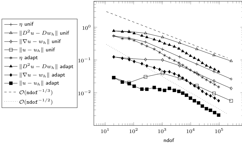
FIGURE 4. Convergence history for Experiment 2.
