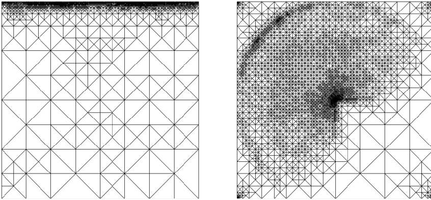
FIGURE 3. Adaptive meshes. Left: Experiment 1, 2 905 vertices, 10 932 degrees of freedom, level 36. Right: Experiment 2; 3 431 vertices, 13 464 degrees of freedom, level 16.
