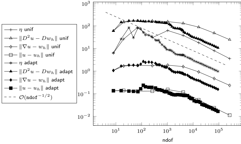
FIGURE 2. Convergence history for Experiment 1.
