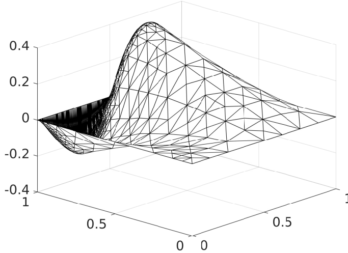
FIGURE 1. Discrete solution u_h for Experiment 1; 2 905 vertices, 10 932 degrees of freedom, level 36.
