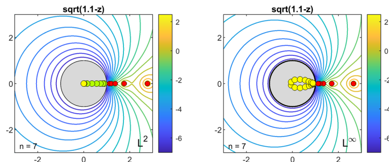
Fig. 8 Potential contours for degree 7 approximations of \sqrt{1.1-z} , following Figure 3. In each case two of the seven poles \{\pi_k\} are off-scale to the right
