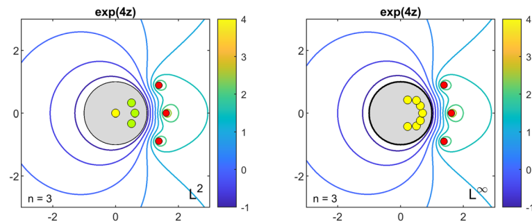
Fig. 6 Potential contours for degree 3 approximations of \exp(4z) , following Figure 1. Contours show integer and half-integer levels of \log_{10} |\phi(z)| , with \phi defined by (4.1). Red dots mark poles of the approximant r , yellow dots mark interpolation points where r = f , and green dots marks double (Hermite) interpolation points with r = f and r' = f' . By Theorem 3.2, for L^2 approximation there is a yellow dot at the origin and green dots at the points of reflection of the red dots in the unit circle
