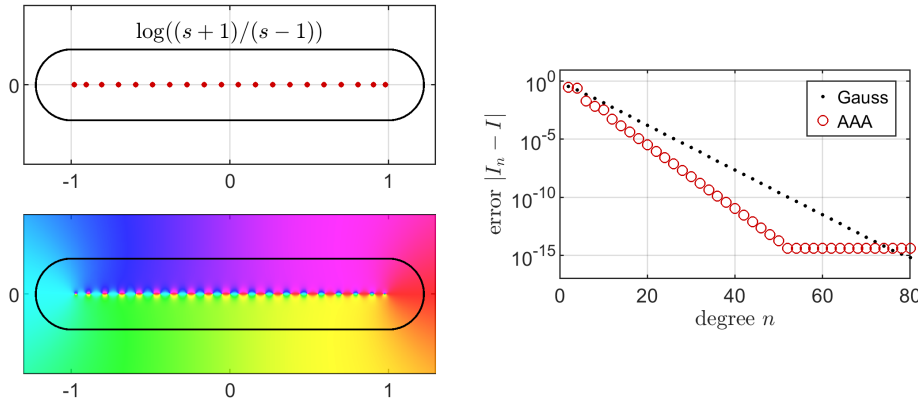
FIG. 3. Variant of Figure 2 in which \log((s+1)/(s-1)) is approximated on an \varepsilon -neighborhood of [-1, 1] rather than a Bernstein ellipse. For the same test integrand as before, the convergence is now faster by a factor of about \pi/2 , and the quadrature nodes are more evenly spaced.
