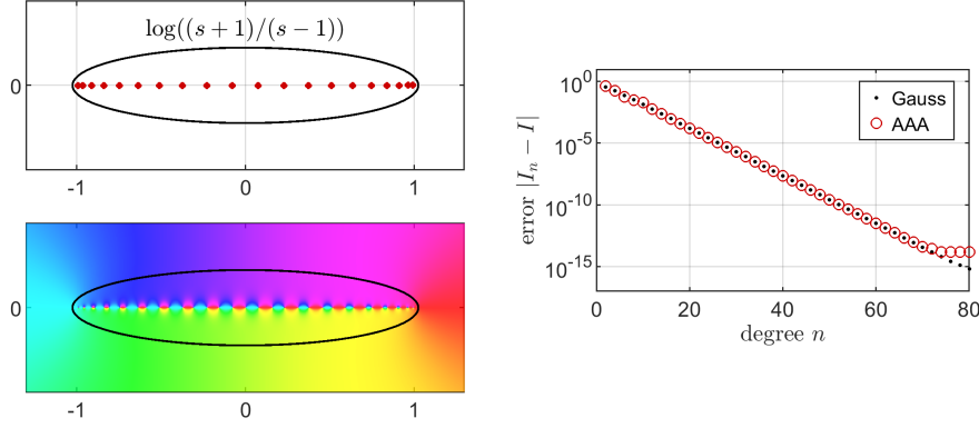
FIG. 2. Quadrature by AAA rational approximation of 2\pi i C(s) = \log((s+1)/(s-1)) on the Bernstein ellipse passing through the singularities at \pm i/\sqrt{20} of the test integrand f(z) = 1/(1+20z^2) on [-1, 1] . The upper-left image shows AAA poles for degree n = 20 , close to the Gauss quadrature nodes of the same degree, and the lower-left image is a phase portrait of the AAA approximation r_{20}(z) (red for positive real, cyan for negative real [67]). The right image shows convergence for this integrand as a function of degree n .
