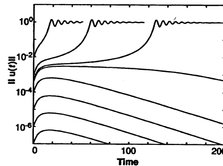
Fig. 10. \|\mathbf{u}(t)\| for solutions to the nonlinear 2 \times 2 model problem of Eq. 14 with initial amplitudes \|\mathbf{u}(0)\| = 10^{-7}, 10^{-6}, 10^{-5}, 10^{-4}, 4 \times 10^{-4}, 5 \times 10^{-4}, 10^{-3}, and 10^{-2} . The threshold amplitude is \|\mathbf{u}(0)\| = 4.22 \times 10^{-4} .
