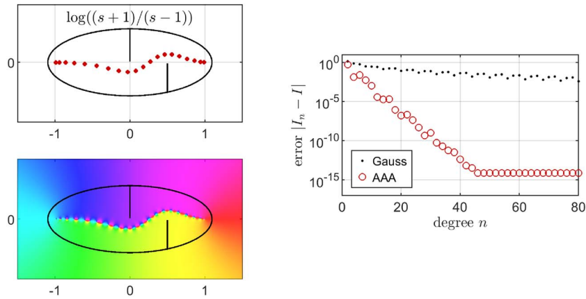
FIG. 5. Variant of Fig. 4 inspired by Hale & Tee (2009) in which there may be several singularities near [-1, 1] , and not just conjugate pairs. The test integrand is \log([z - .01i]i) + \log([z - (.5 - .01i)]i) .
