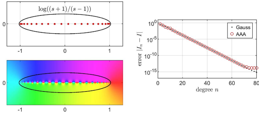
FIG. 2. Quadrature by AAA rational approximation of 2\pi iC(s) = \log((s + 1)/(s - 1)) on the Bernstein ellipse passing through the singularities at \pm i/\sqrt{20} of the test integrand f(z) = 1/(1 + 20z^2) on [-1, 1] . The upper-left image shows AAA poles for degree n = 20 , close to the Gauss quadrature nodes of the same degree, and the lower-left image is a phase portrait of the AAA approximation r_{20}(z) (red for positive real, cyan for negative real (Wegert, 2012)). The right image shows convergence for this integrand as a function of degree n .
