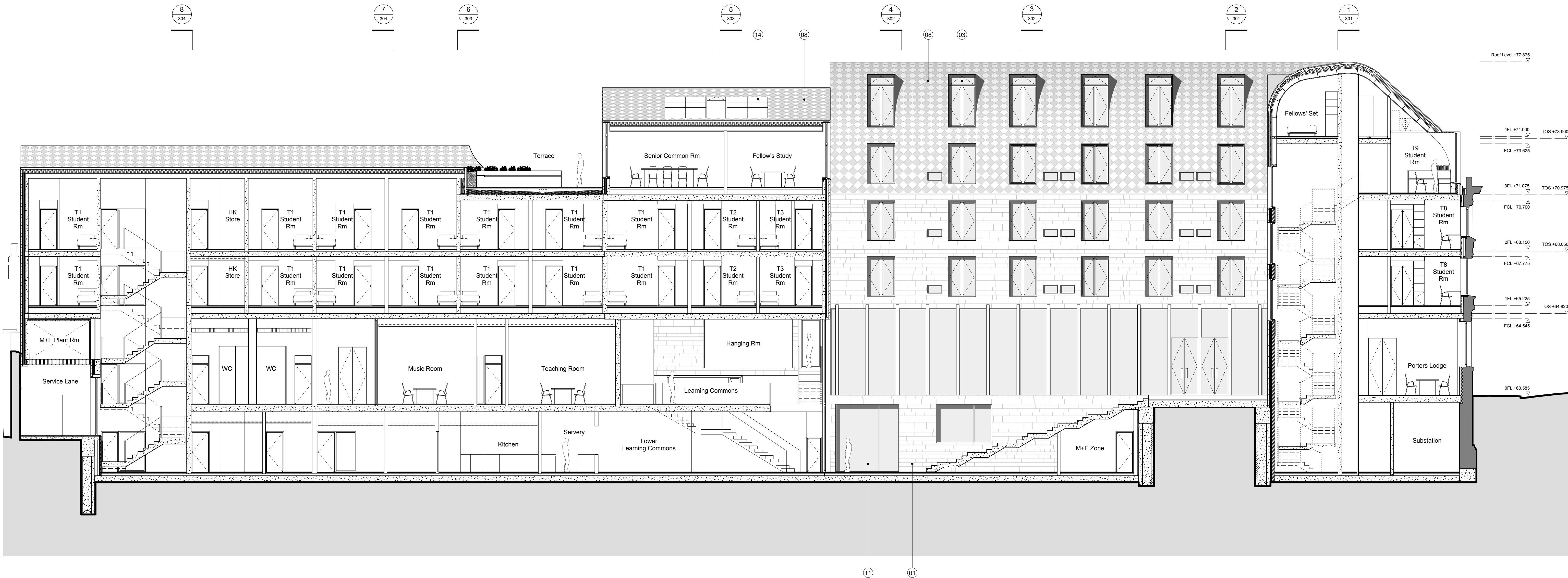
12 LONG SECTION 12
