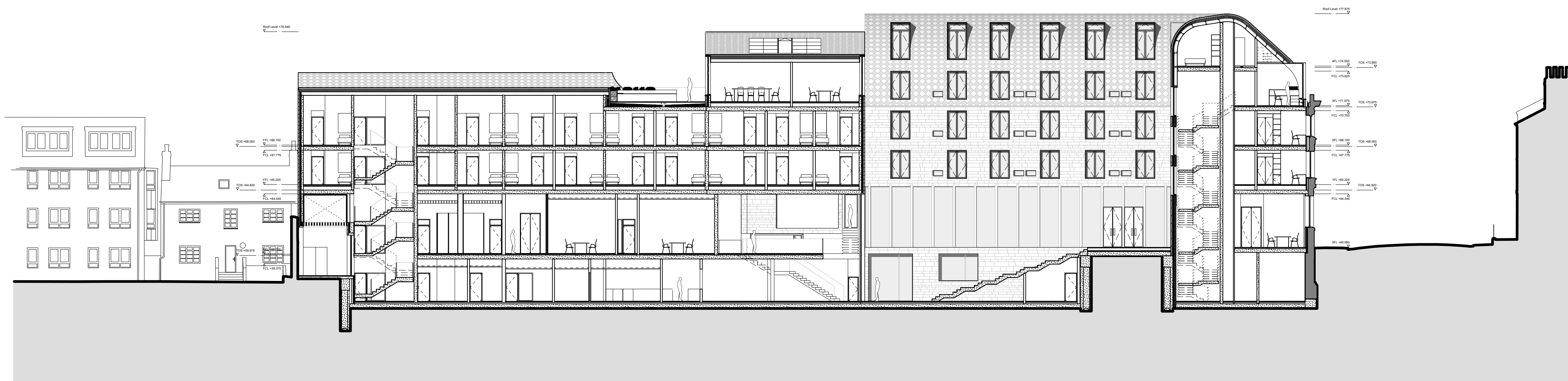
12 LONG SECTION 12
