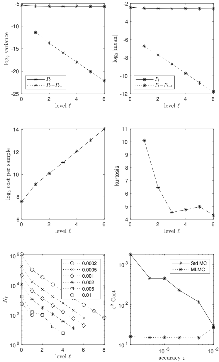
Figure 1: MLMC using adapted timestepping for an SDE with a singular drift
