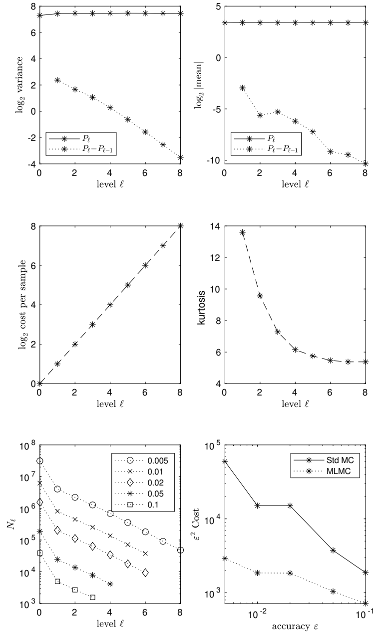
Figure 1: Heston results without antithetic treatment
