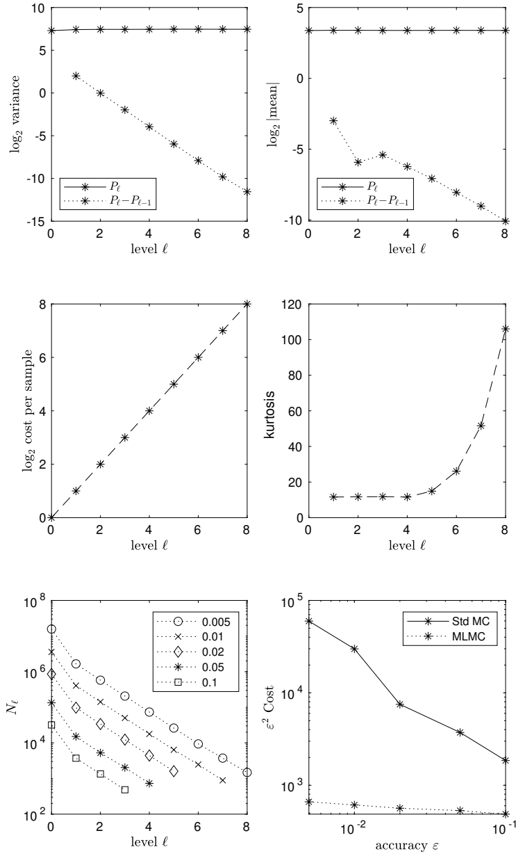
Figure 2: Heston results with antithetic treatment
