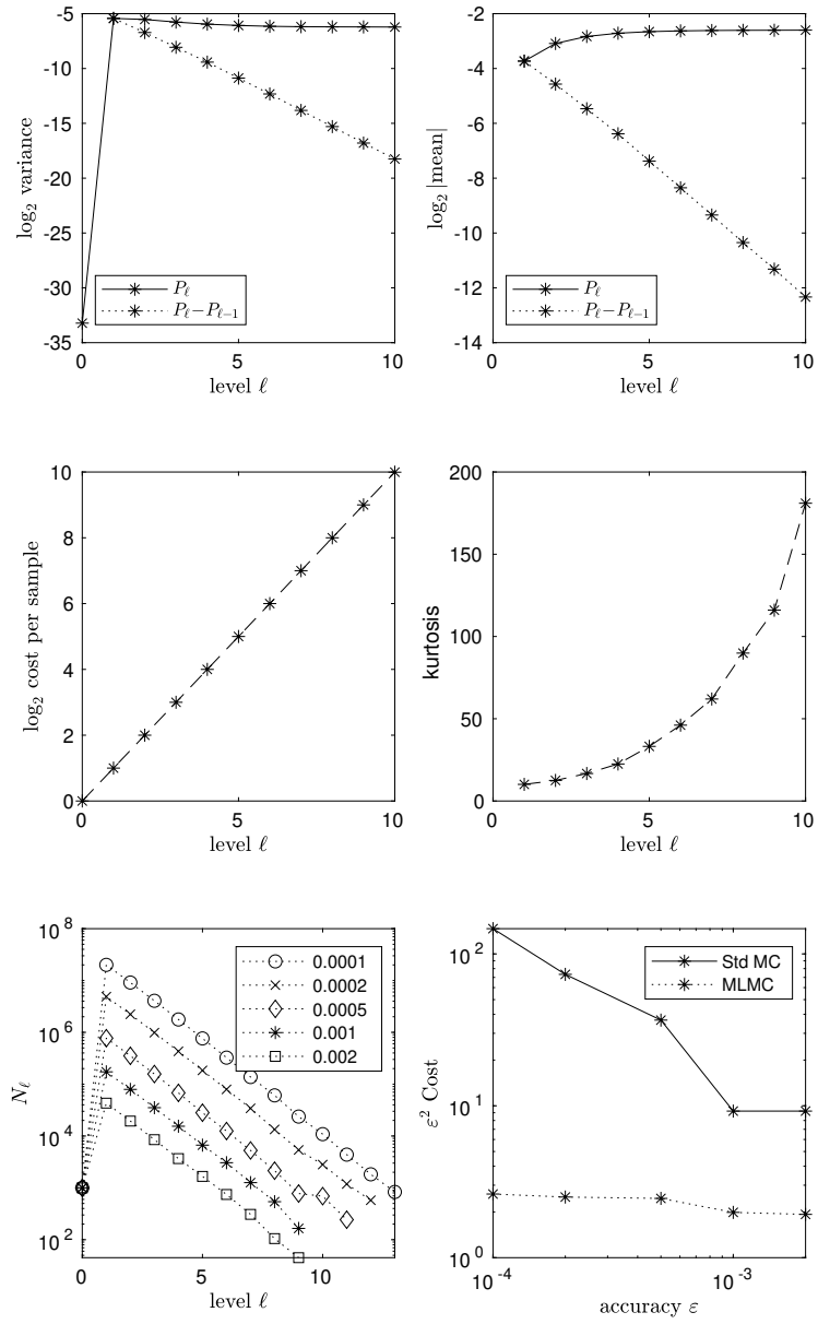
Figure 1: Model test problem from 2019 paper with Takashi Goda
